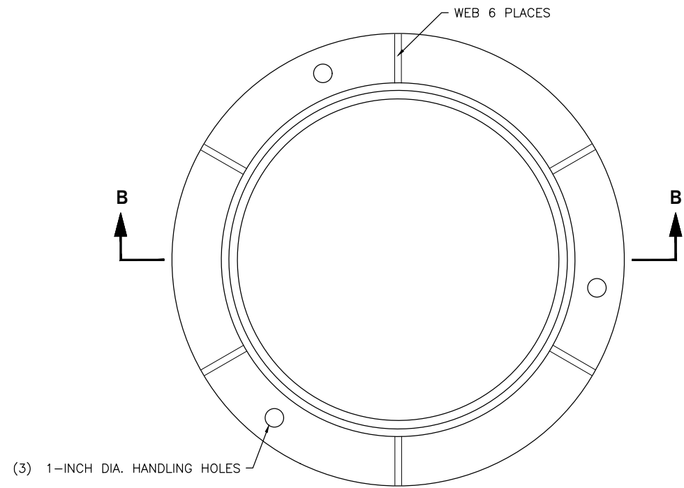
3715Z STACKING GRAY IRON OR DUCTILE IRON FRAME
