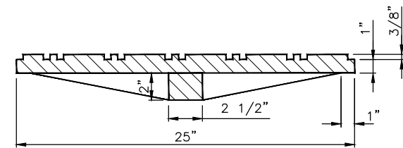
SECTION A-A - GREY IRON OR DUCTILE IRON NON LOCKING COVER MINIMUM WEIGHT 100 LBS.
